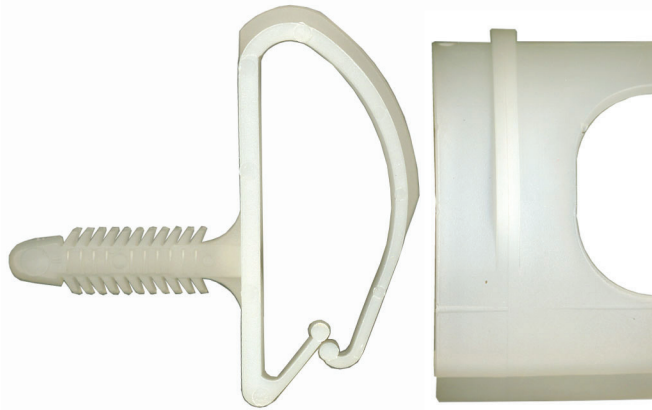
FA 2894 $1.50 Wire Routing Clip Stem 5/16x11/32x1-1/4 Long GM 19810n
